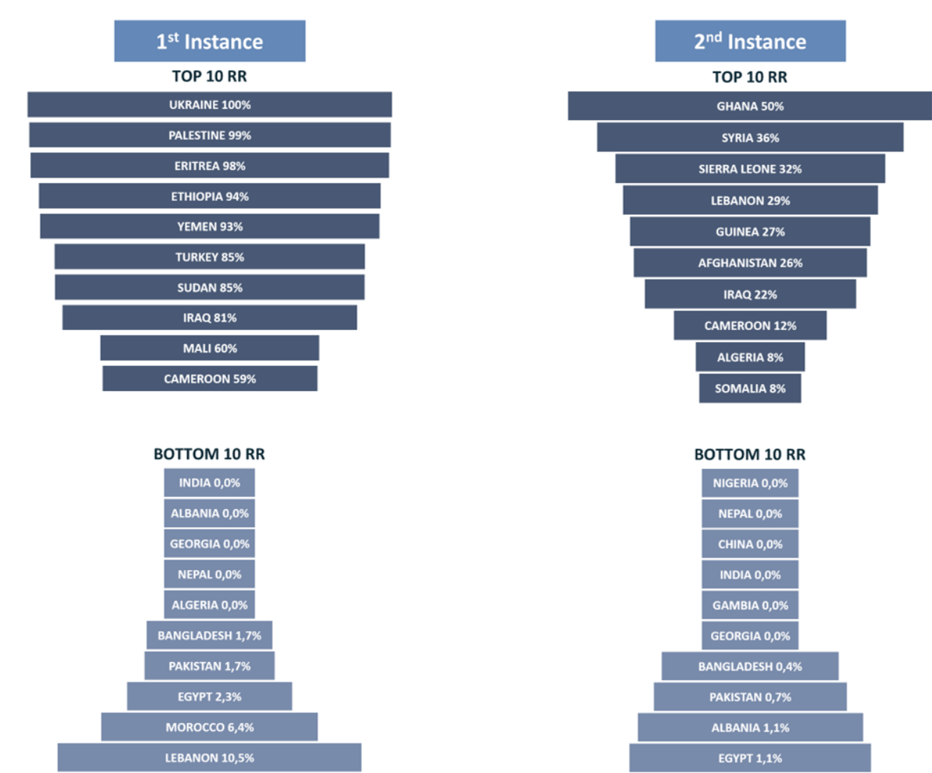
Chart 28. Recognition Rate 2-months 2023 in 1 st & 2 nd Instance for top and bottom 10 nationalities. For the calculation of Recognition rate in 1 st Instance have been included nationalities for which have been issued at least 10 decisions in 2023 and for the 2 nd Instance at least 10 decisions. See Appendix Table 12g
